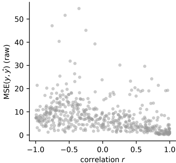
raw MSE conflates r with scale
