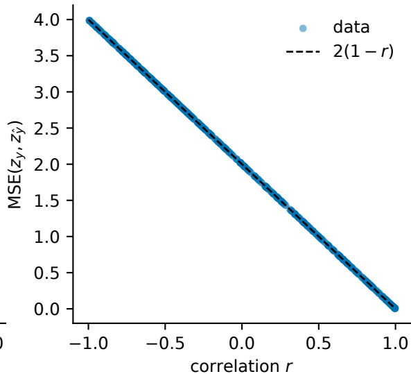
standardized MSE = 2(1 - r)
